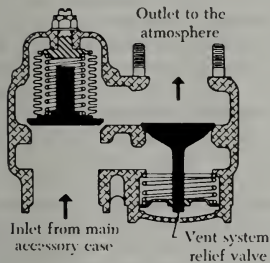
(B) Sectional view of breather pressurizing valve
